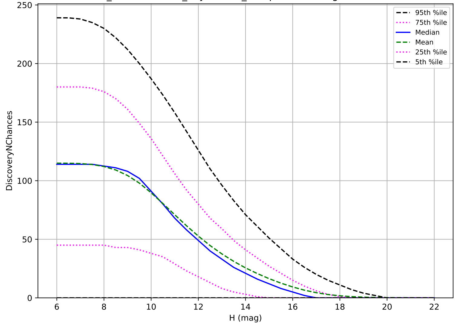
weather_cloudso10v3.4_10yrs: OCC_r5 3 pairs in 15 nights detection loss
