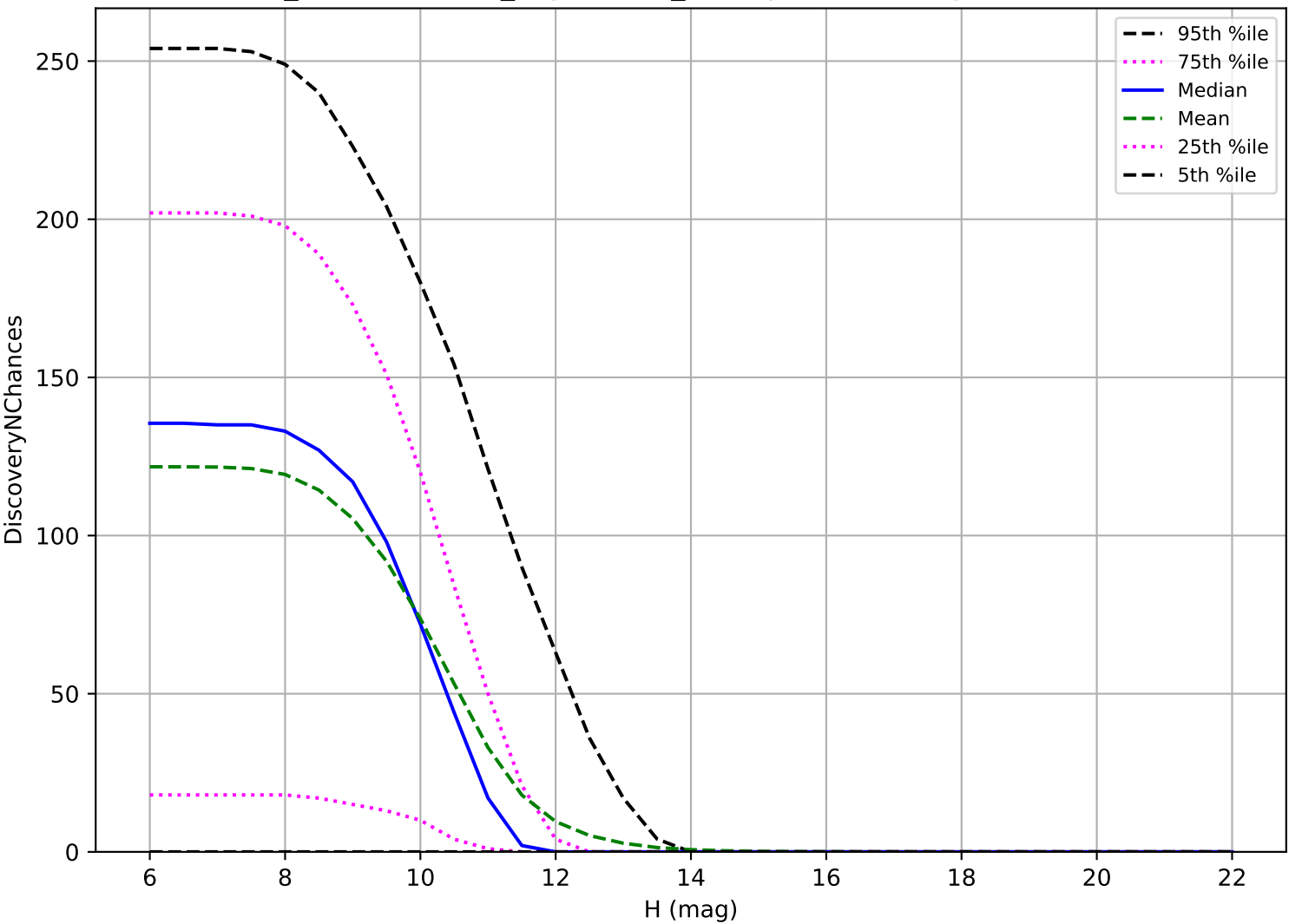
weather_cloudso10v3.4_10yrs: OCC_r20 3 pairs in 15 nights detection loss
