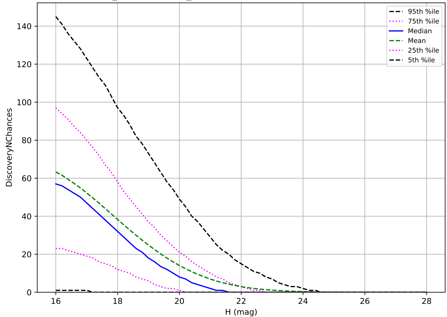
weather_cloudso10v3.4_10yrs: NEO 3 pairs in 15 nights detection loss
