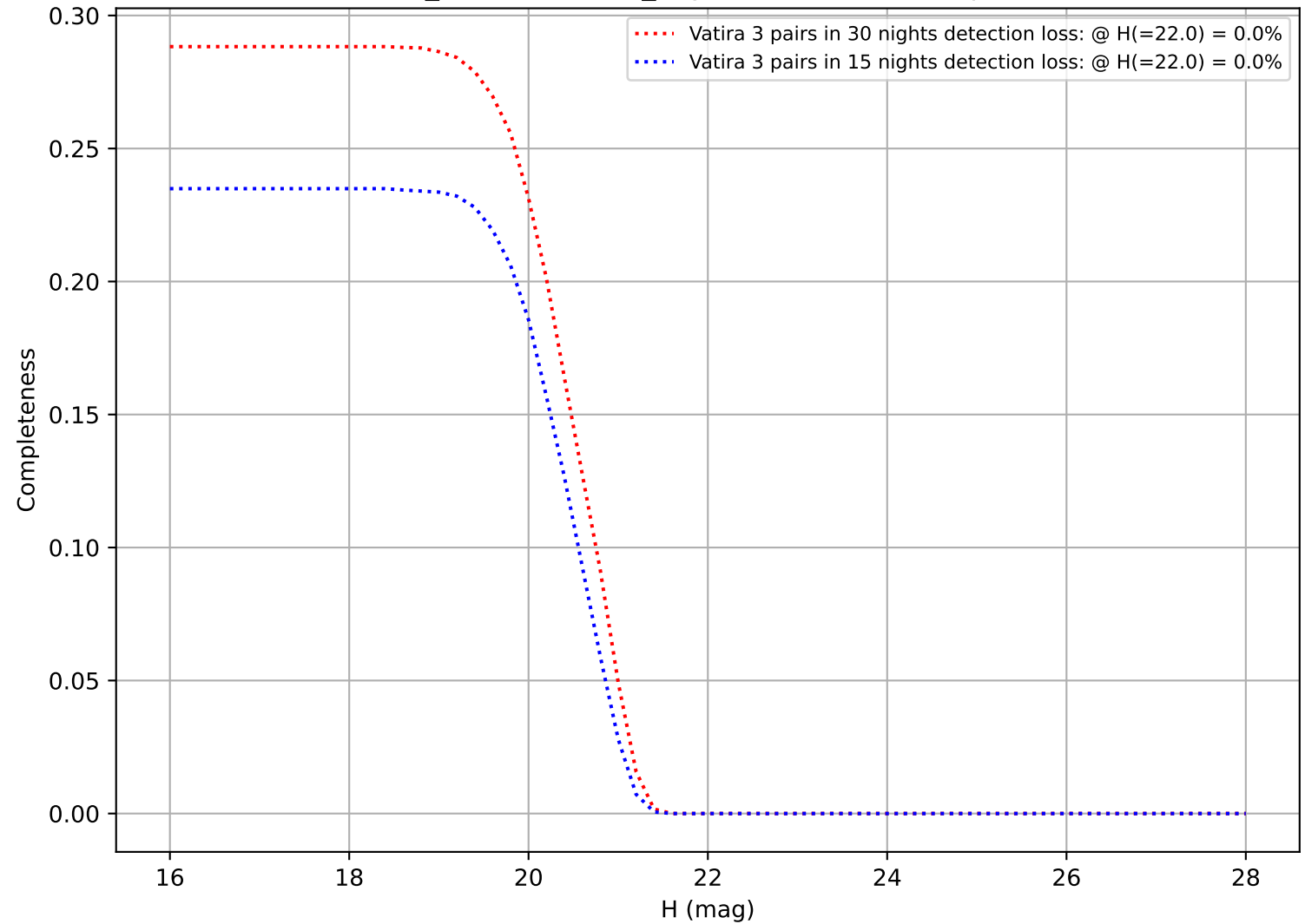
weather_cloudso10v3.4_10yrs: DifferentialCompleteness
