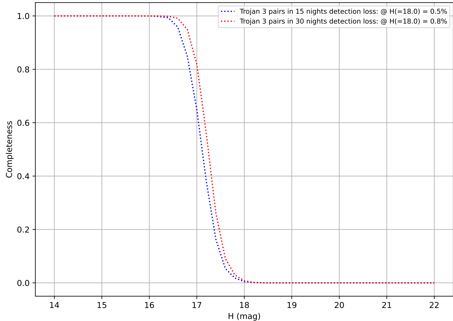
weather_cloudso10v3.4_10yrs: DifferentialCompleteness
