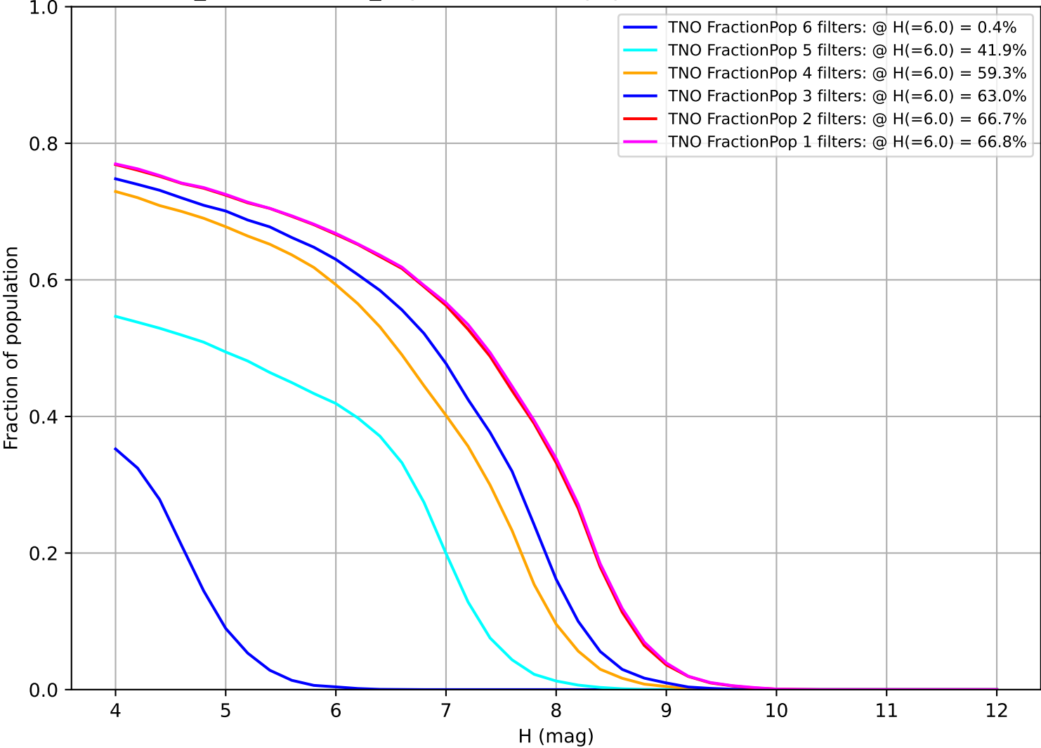
weather_cloudso10v3.4_10yrs: Fraction of population with colors in X filters TNO
