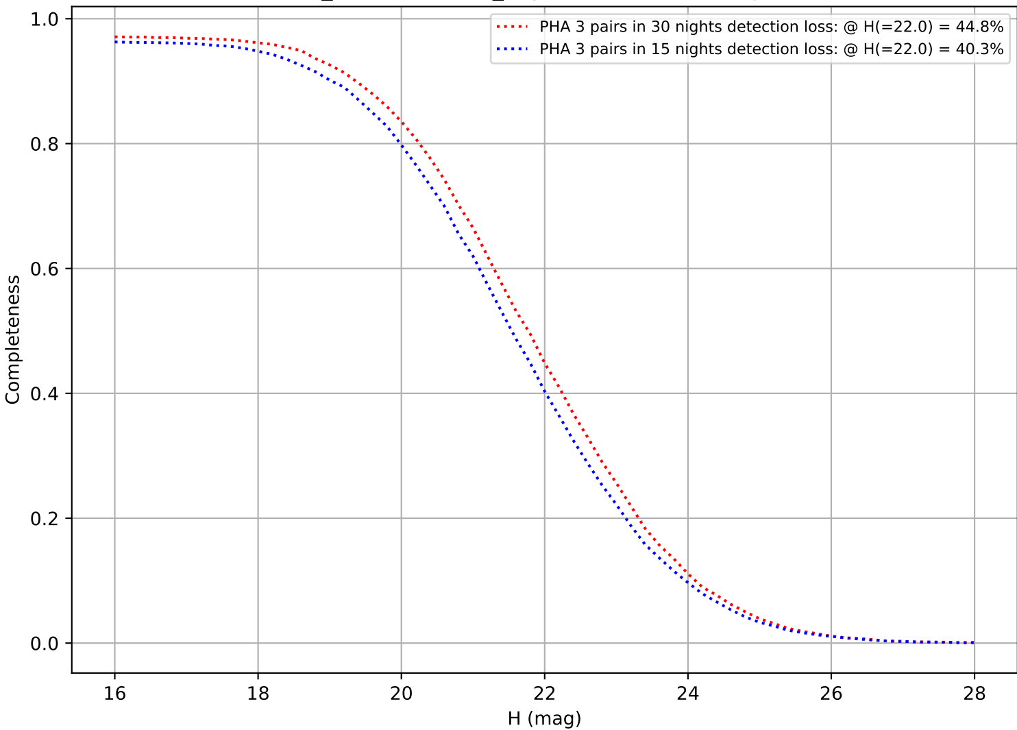
weather_cloudso10v3.4_10yrs: DifferentialCompleteness
