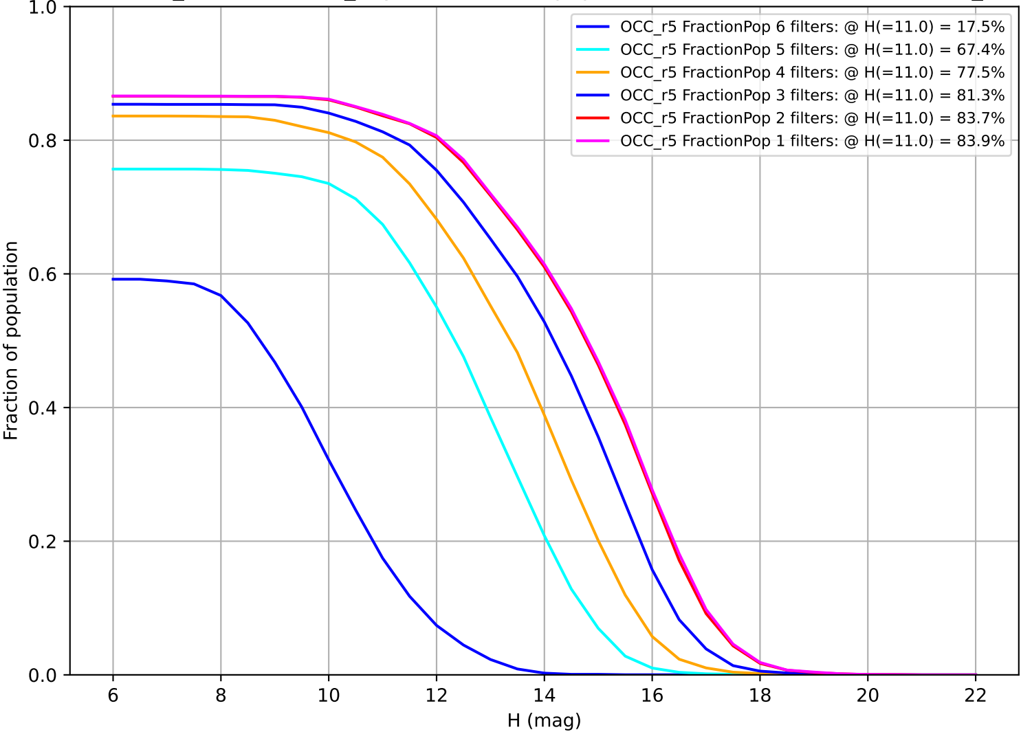
weather_cloudso10v3.4_10yrs: Fraction of population with colors in X filters OCC_r5
