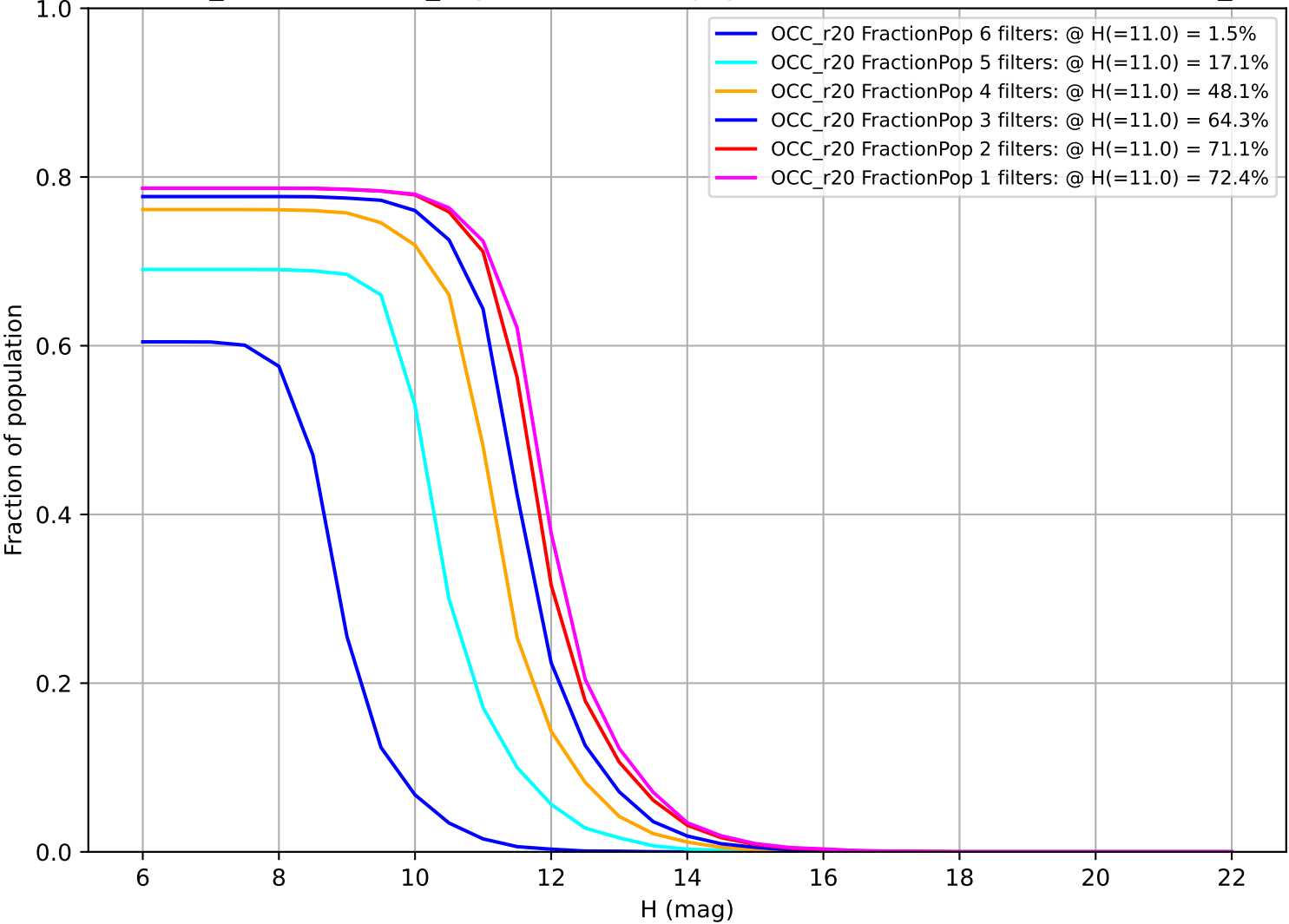
weather_cloudso10v3.4_10yrs: Fraction of population with colors in X filters OCC_r20
