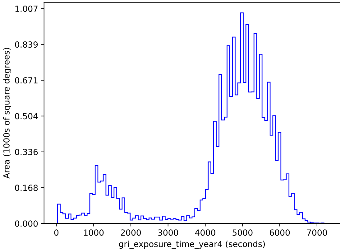
weather_cloudso10v3.4_10yrs gri band non-DD: gri_exposure_time_year4
