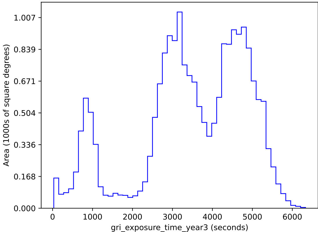
weather_cloudso10v3.4_10yrs gri band non-DD: gri_exposure_time_year3
