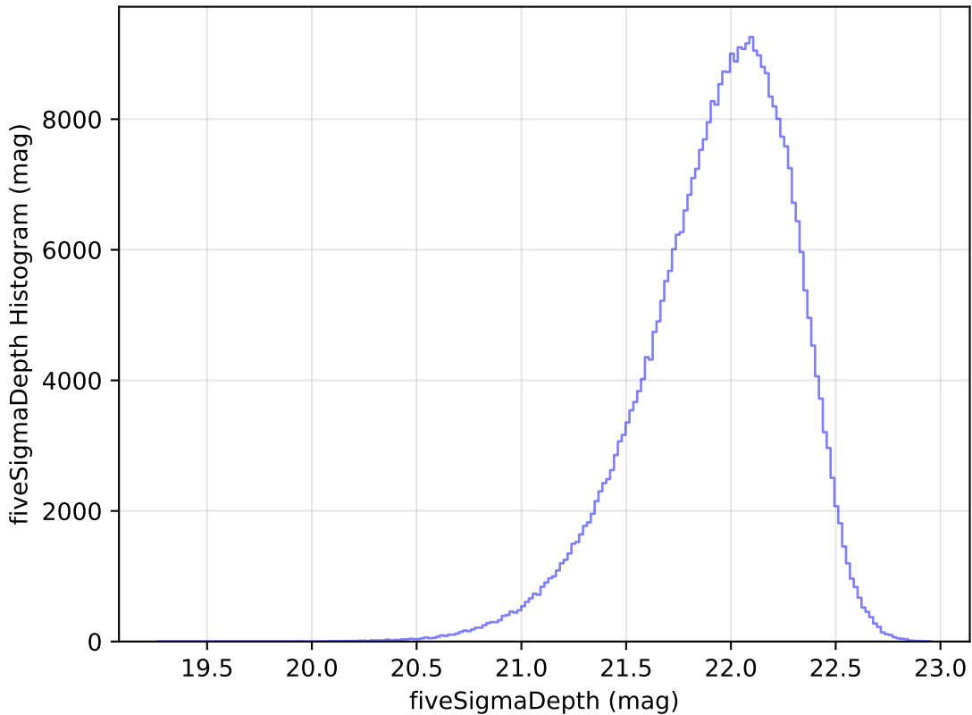
weather_cloudso10v3.4_10yrs y: fiveSigmaDepth Histogram
