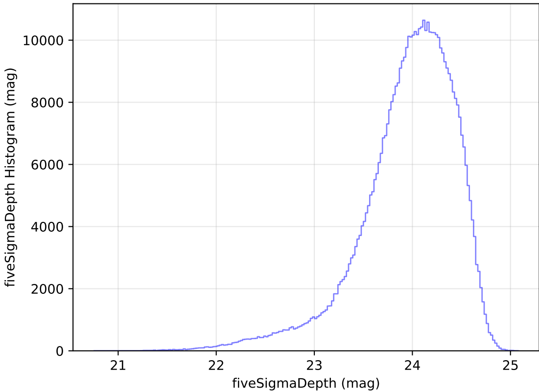
weather_cloudso10v3.4_10yrs r: fiveSigmaDepth Histogram
