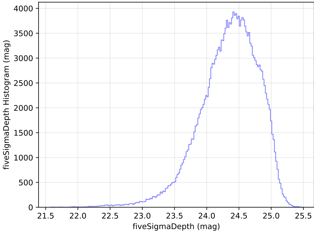
weather_cloudso10v3.4_10yrs g: fiveSigmaDepth Histogram
