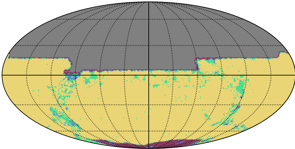
weather_cloudso10v3.4_10yrs y band: YearCoverage night
