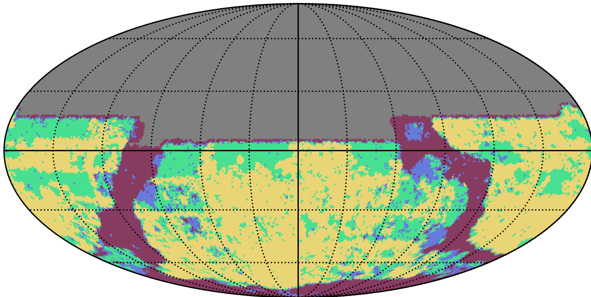
weather_cloudso10v3.4_10yrs u band: YearCoverage night
