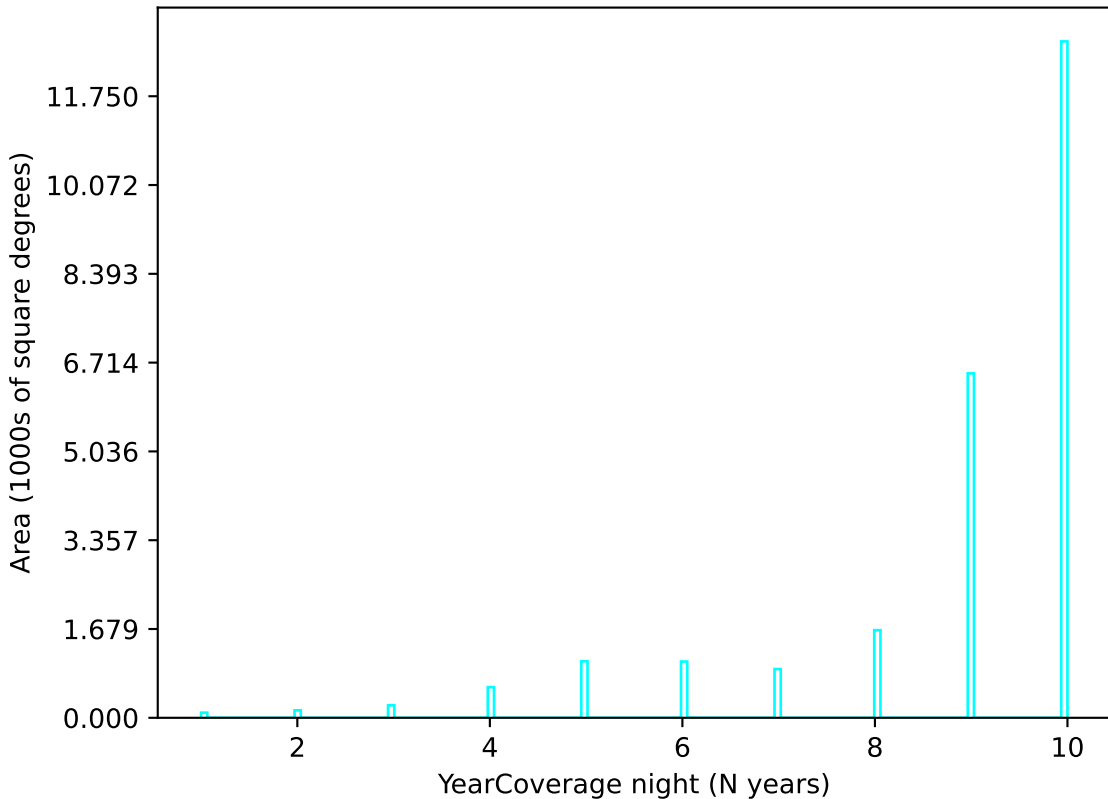
weather_cloudso10v3.4_10yrs u band: YearCoverage night
