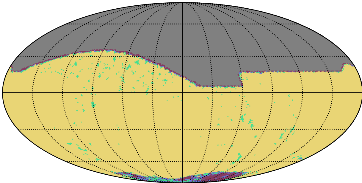
weather_cloudso10v3.4_10yrs r band: YearCoverage night
