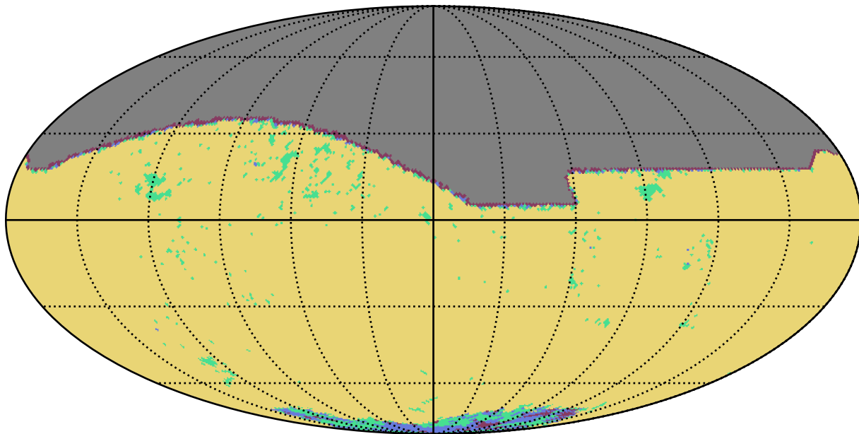
weather_cloudso10v3.4_10yrs i band: YearCoverage night
