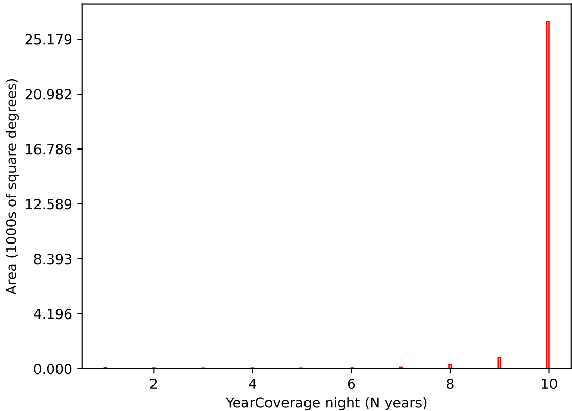
weather_cloudso10v3.4_10yrs i band: YearCoverage night
