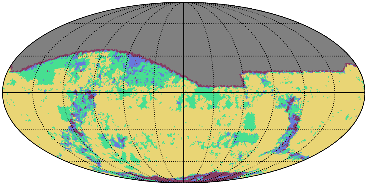
weather_cloudso10v3.4_10yrs g band: YearCoverage night
