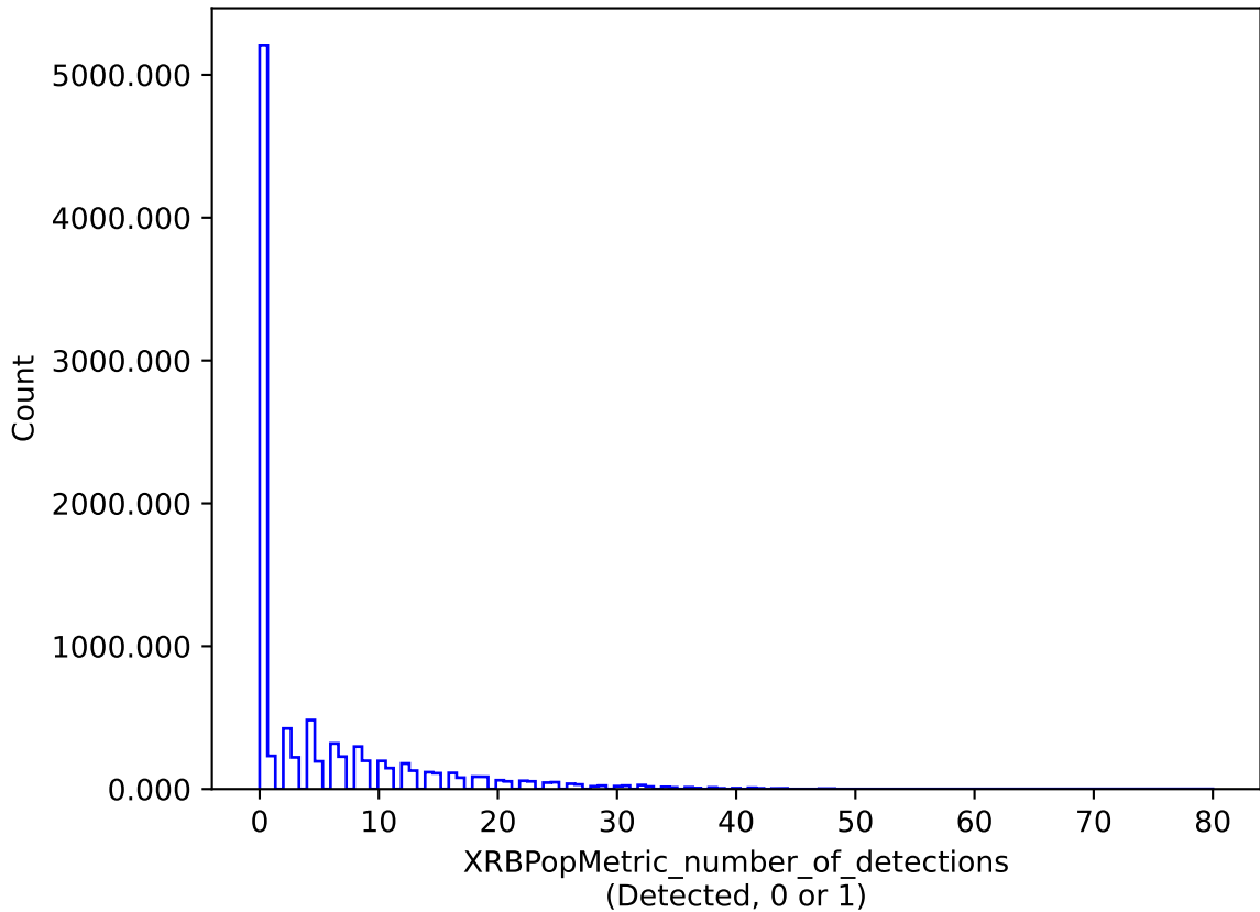
weather_cloudso10v3.4_10yrs : XRBPoMetric_number_of_detections
