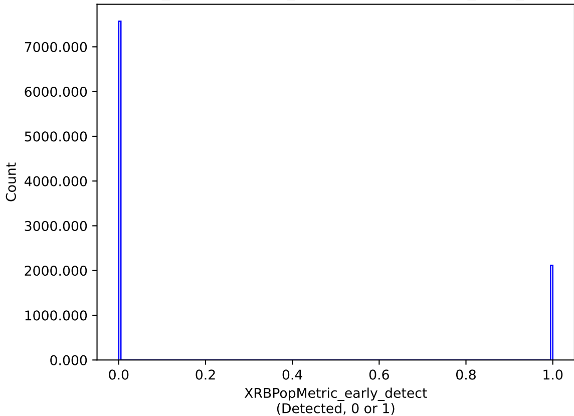
weather_cloudso10v3.4_10yrs : XRBPoMetric_early_detect
