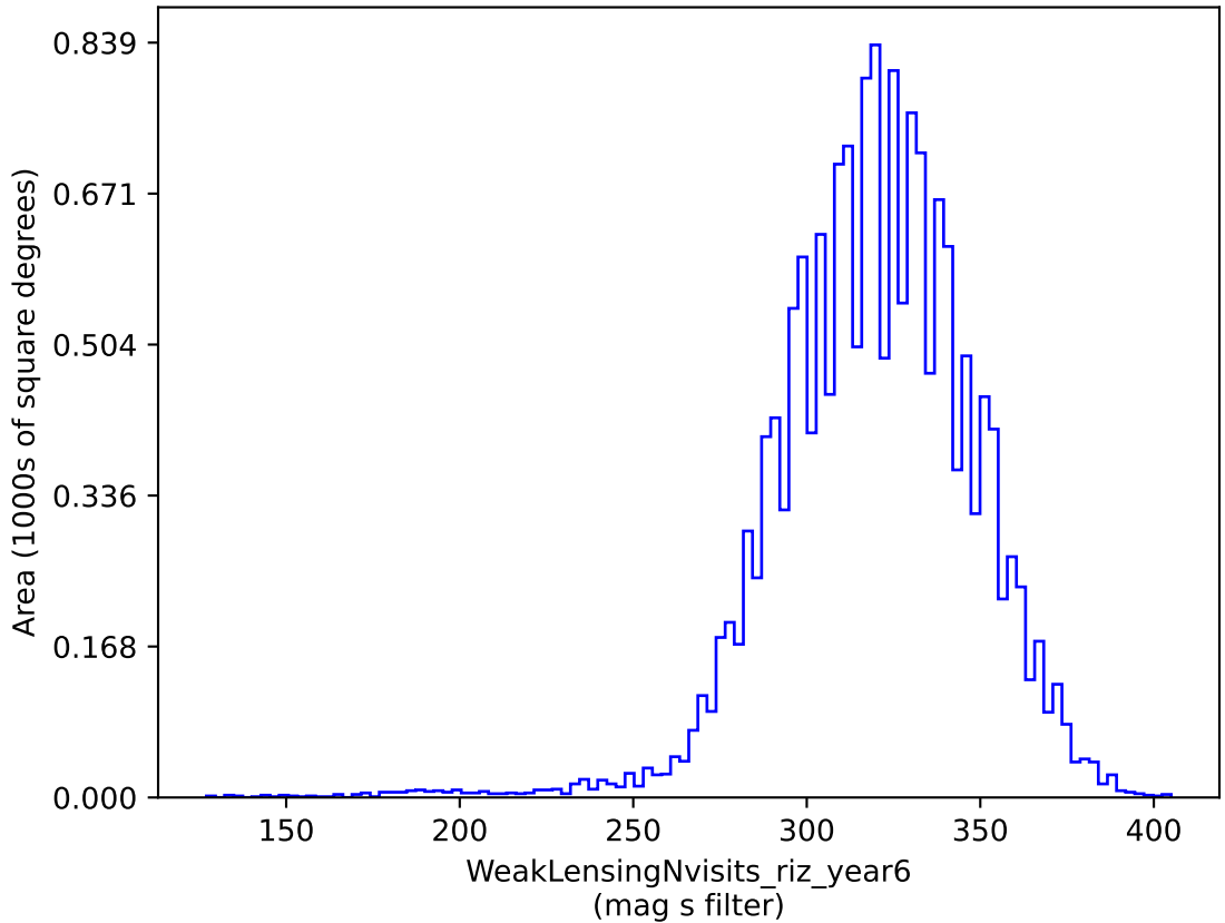
weather_cloudso10v3.4_10yrs gri band non-DD: WeakLensingNvisits_riz_year6
