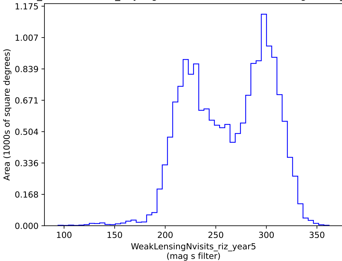
weather_cloudso10v3.4_10yrs gri band non-DD: WeakLensingNvisits_riz_year5
