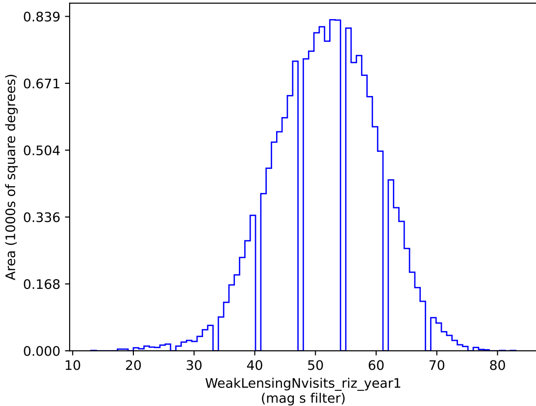
weather_cloudso10v3.4_10yrs gri band non-DD: WeakLensingNvisits_riz_year1
