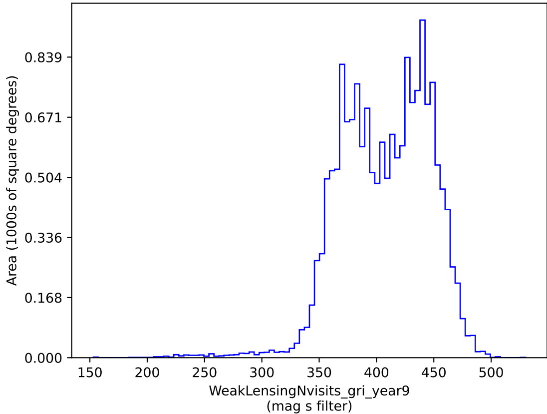
weather_cloudso10v3.4_10yrs gri band non-DD: WeakLensingNvisits_gri_year9
