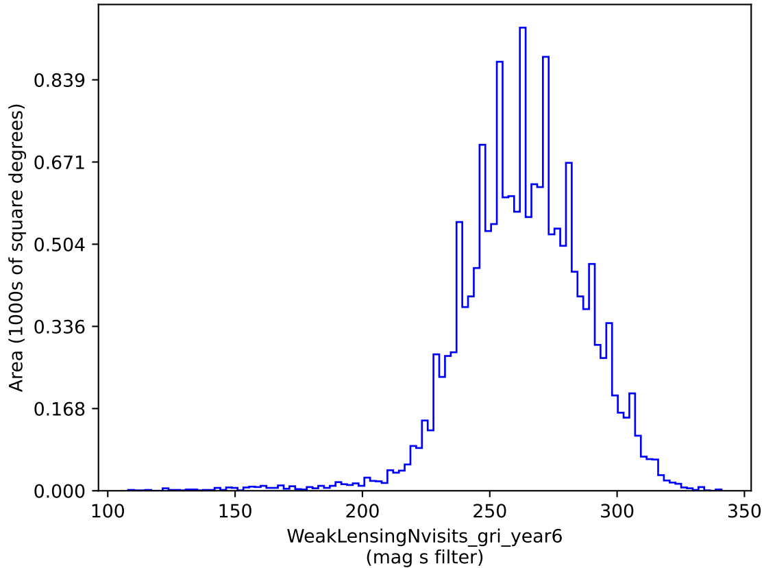
weather_cloudso10v3.4_10yrs gri band non-DD: WeakLensingNvisits_gri_year6
