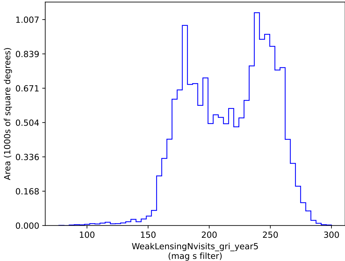
weather_cloudso10v3.4_10yrs gri band non-DD: WeakLensingNvisits_gri_year5
