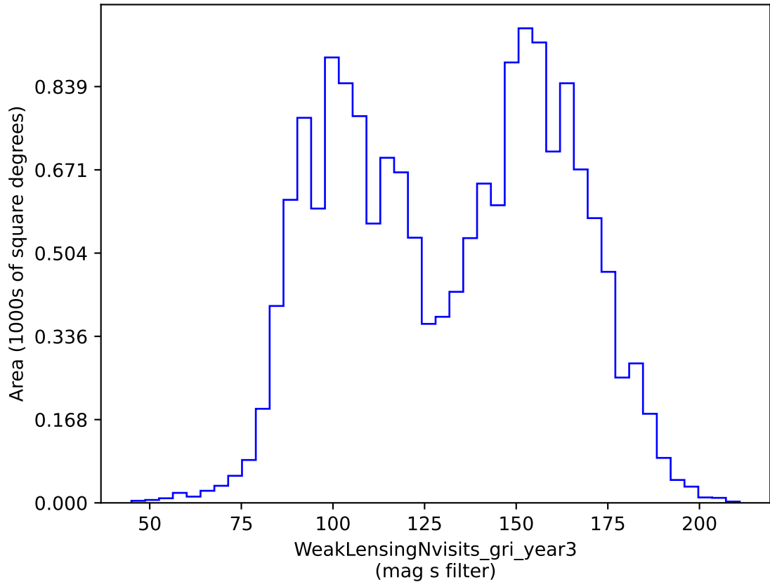
weather_cloudso10v3.4_10yrs gri band non-DD: WeakLensingNvisits_gri_year3
