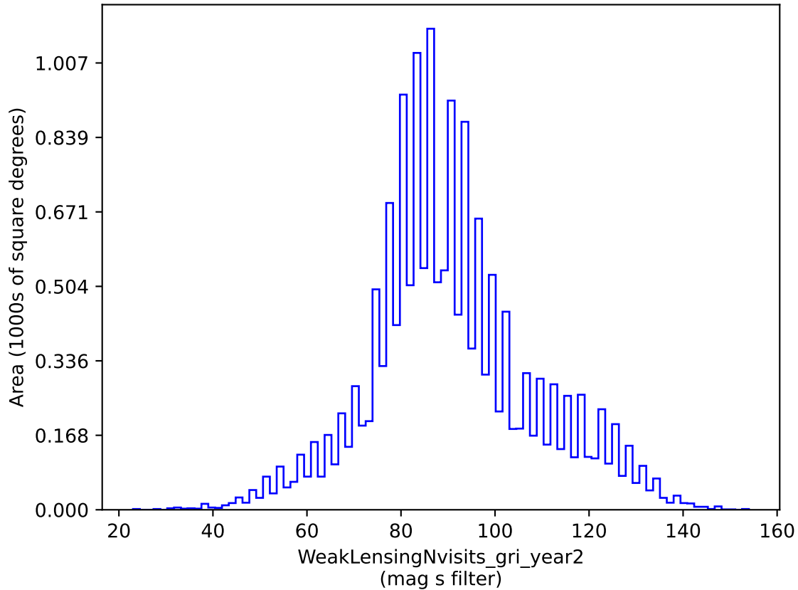
weather_cloudso10v3.4_10yrs gri band non-DD: WeakLensingNvisits_gri_year2
