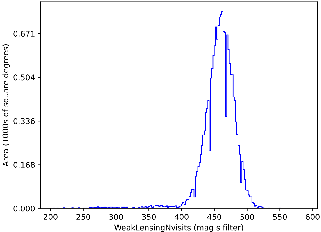
weather_cloudso10v3.4_10yrs gri band non-DD: WeakLensingNvisits
