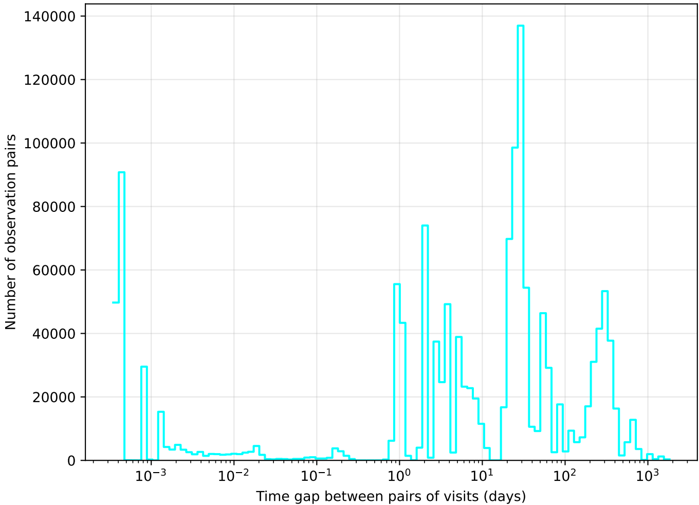
weather_cloudso10v3.4_10yrs u band: Tgaps observationStartMJD
