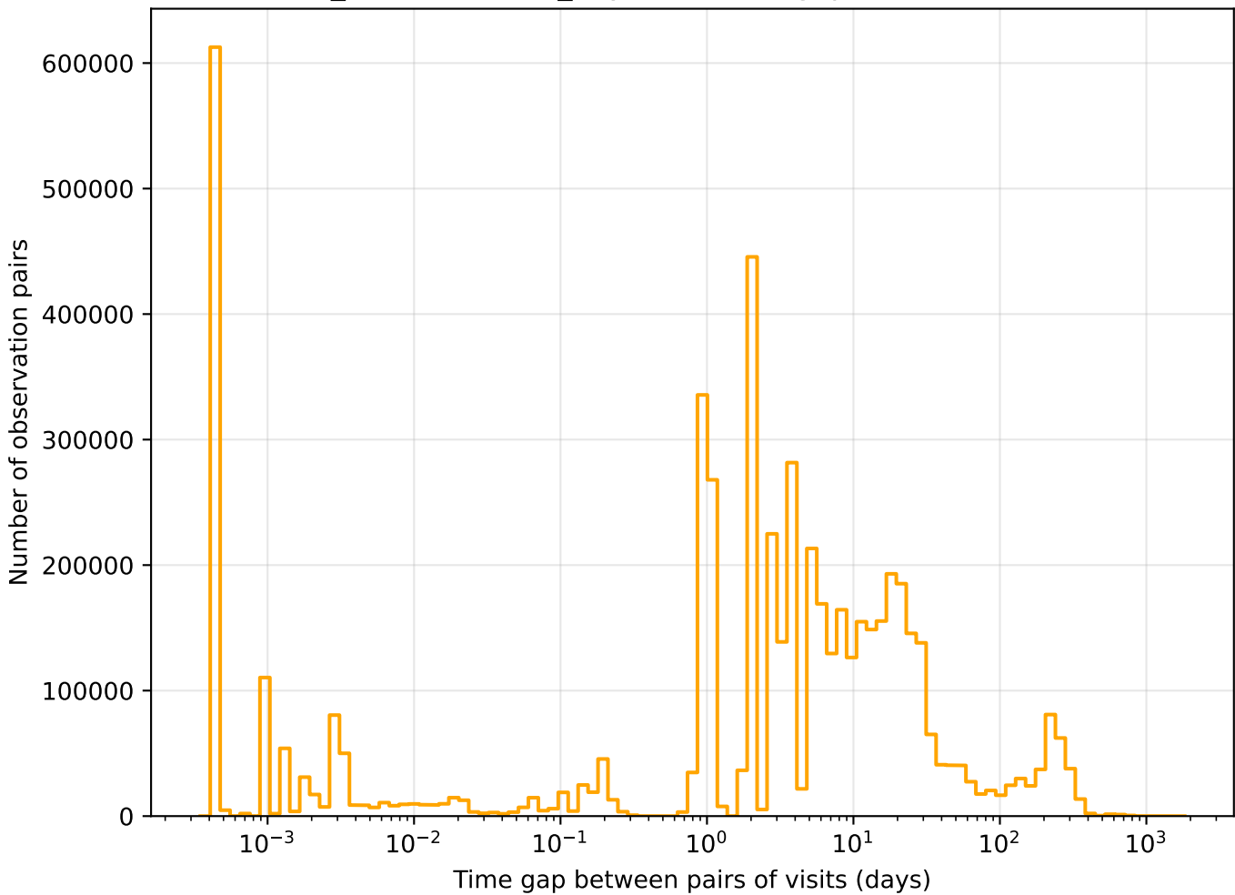
weather_cloudso10v3.4_10yrs r band: Tgaps observationStartMJD
