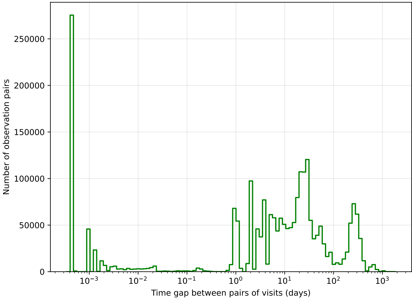
weather_cloudso10v3.4_10yrs g band: Tgaps observationStartMJD
