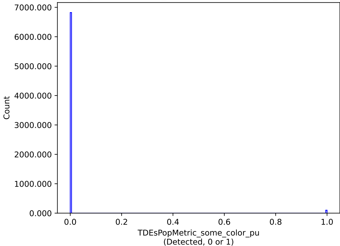
weather_cloudso10v3.4_10yrs : TDEsPopMetric_some_color_pu
