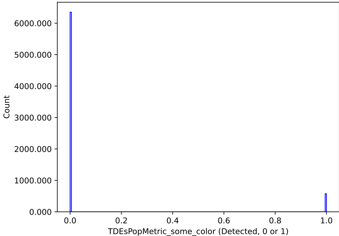
weather_cloudso10v3.4_10yrs : TDEsPopMetric_some_color
