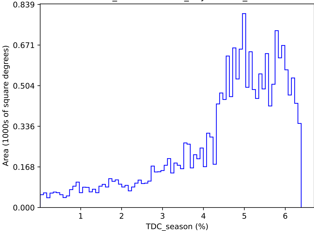
weather_cloudso10v3.4_10yrs : TDC_season
