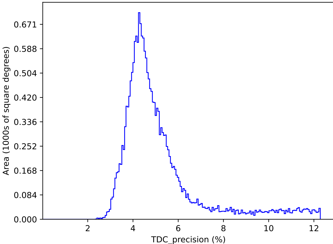
weather_cloudso10v3.4_10yrs : TDC_precision
