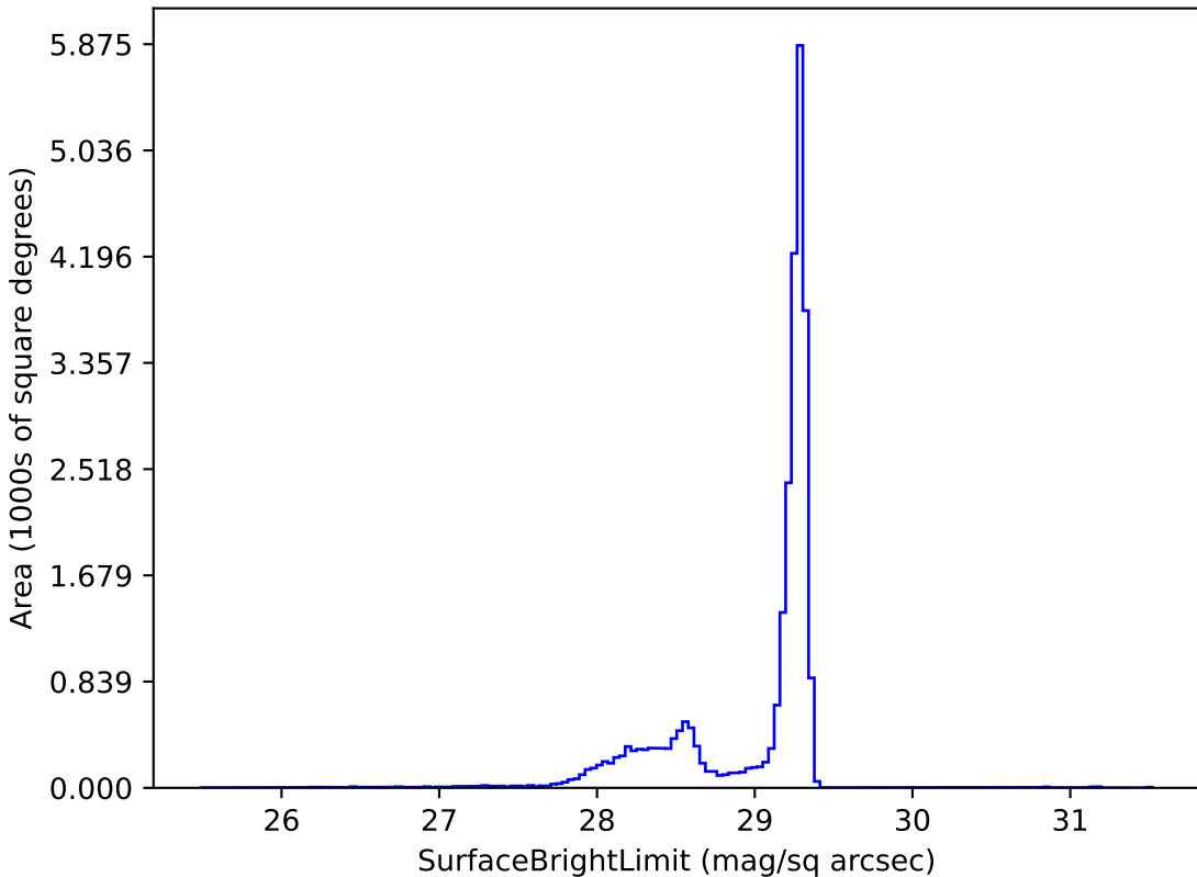
weather_cloudso10v3.4_10yrs z: SurfaceBrightLimit
