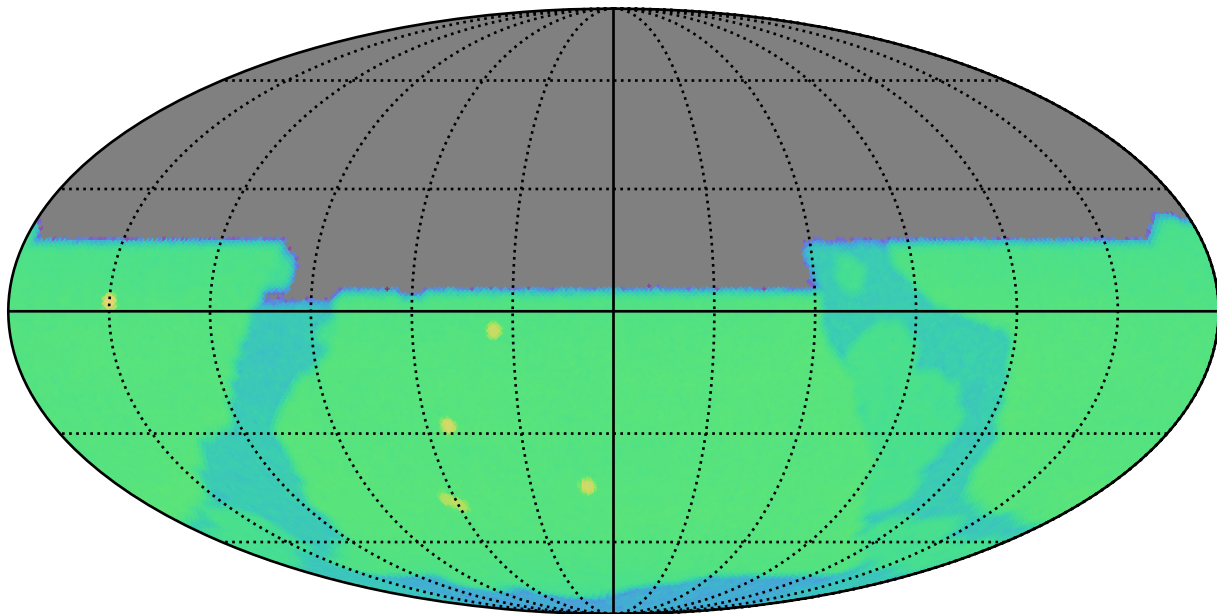
weather_cloudso10v3.4_10yrs y: SurfaceBrightLimit
