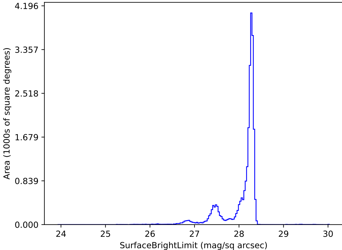
weather_cloudso10v3.4_10yrs y: SurfaceBrightLimit
