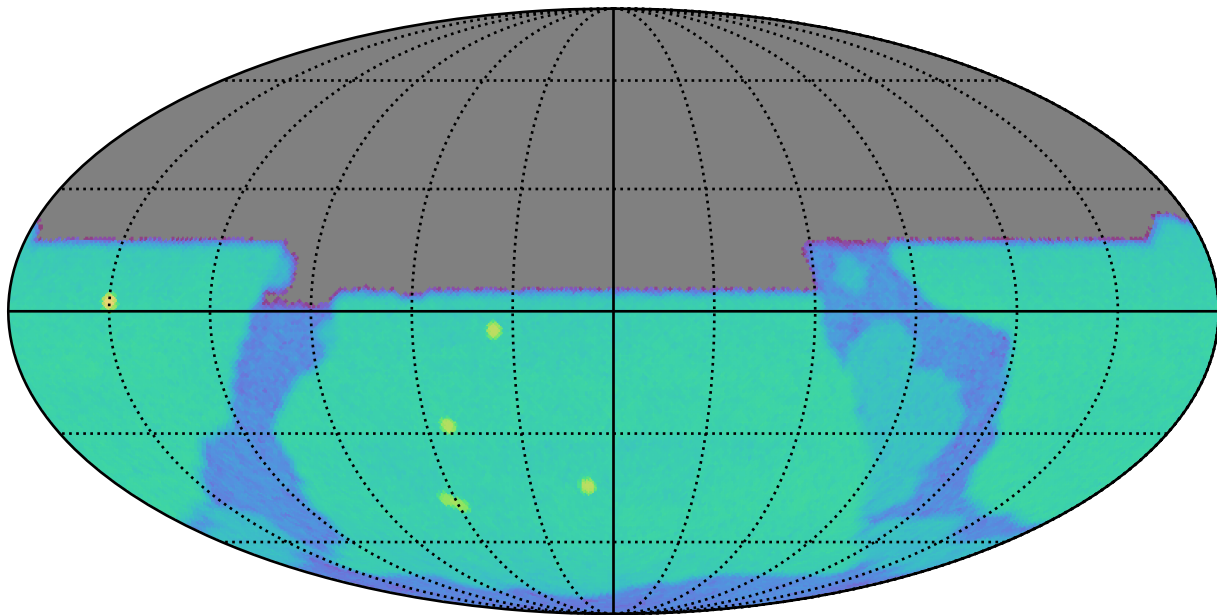
weather_cloudso10v3.4_10yrs u: SurfaceBrightLimit
