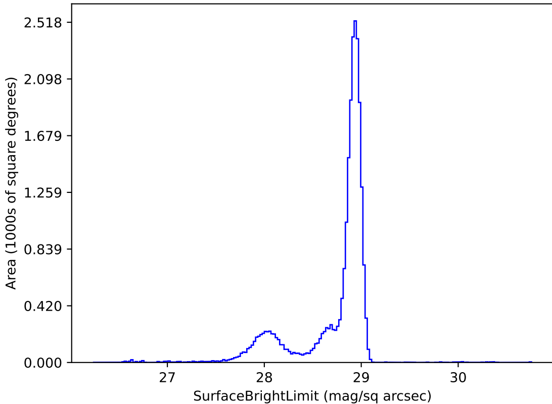
weather_cloudso10v3.4_10yrs u: SurfaceBrightLimit
