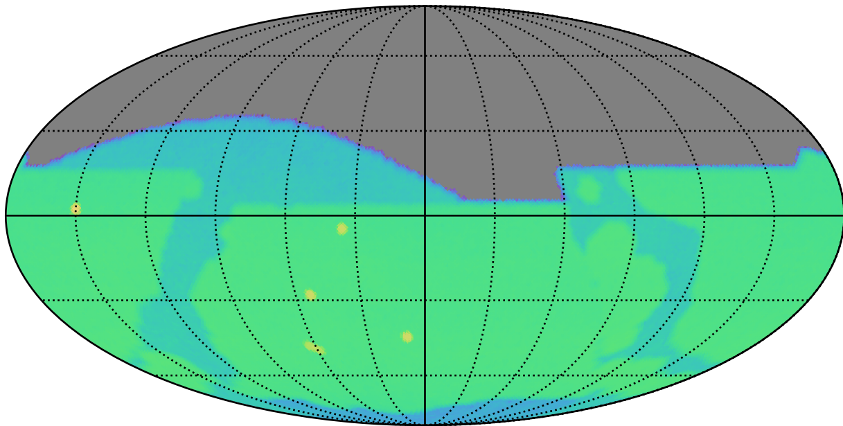
weather_cloudso10v3.4_10yrs r: SurfaceBrightLimit
