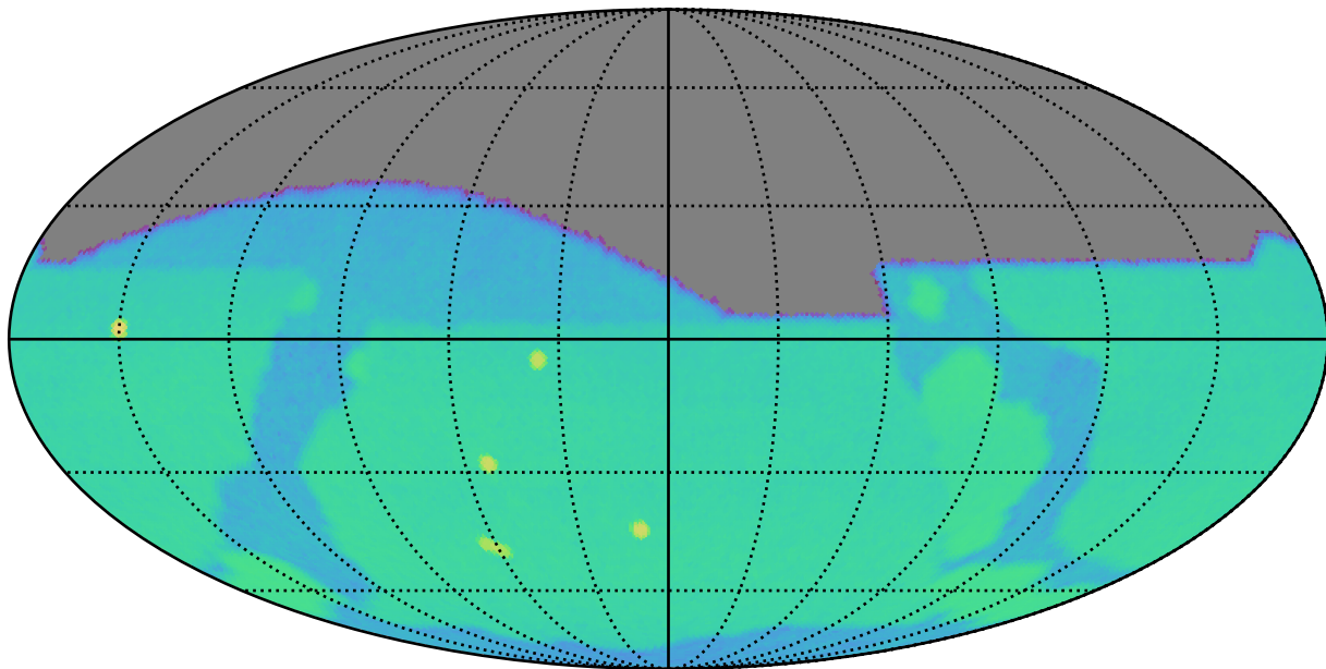
weather_cloudso10v3.4_10yrs g: SurfaceBrightLimit
