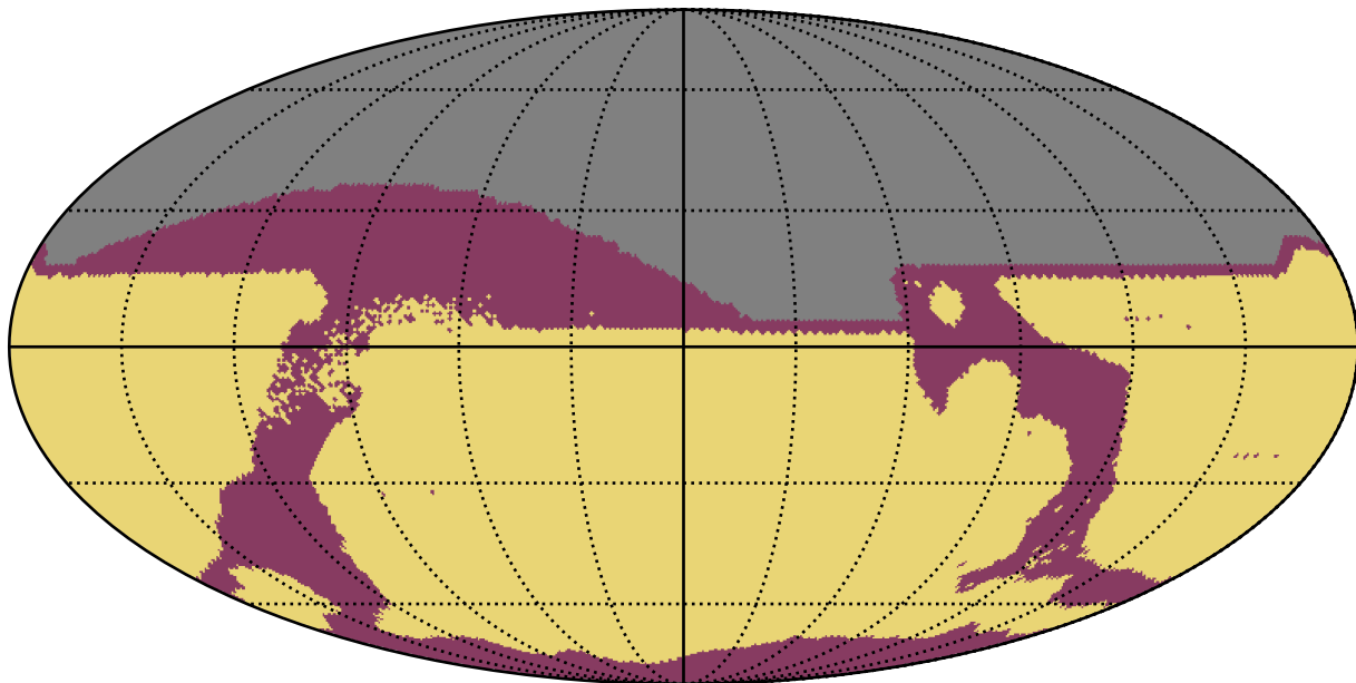
weather_cloudso10v3.4_10yrs : RapidRevisits
