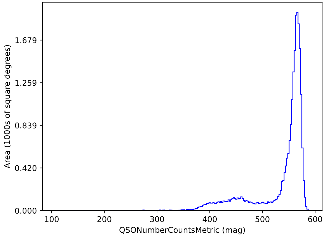
weather_cloudso10v3.4_10yrs y band and non-DD: QSONumberCountsMetric
