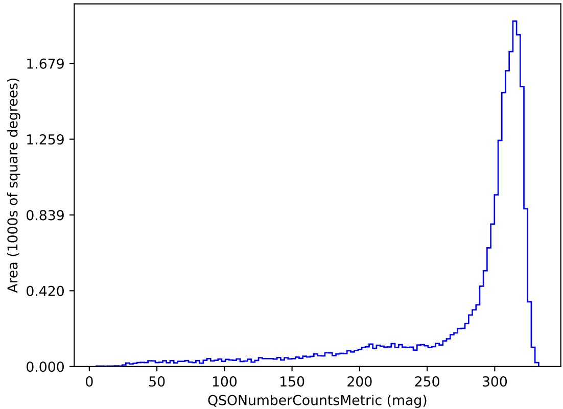
weather_cloudso10v3.4_10yrs u band and non-DD: QSONumberCountsMetric
