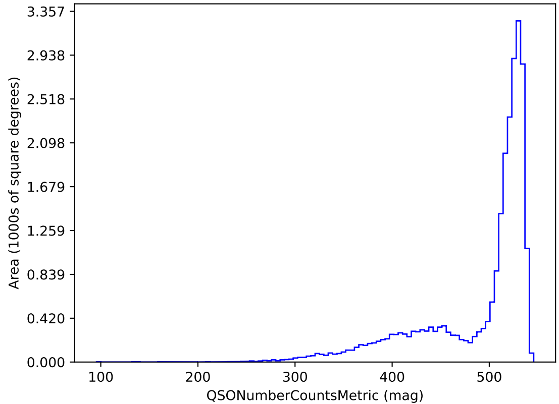
weather_cloudso10v3.4_10yrs r band and non-DD: QSONumberCountsMetric
